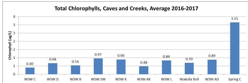
Figure 2.11: Chlorophylls, the green photosynthetic pigments of plants and algae, were sampled for the caves flowing to Wakulla Springs as part of Phase II. MLI data.
