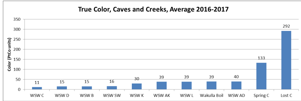
Figure 2.10: True Color was sampled for the caves flowing to Wakulla Springs as part of Phase II. MLI data.
