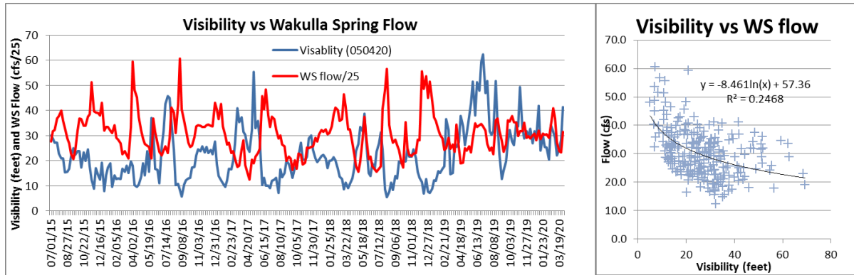
Figure 4.2: Weekly visibility and regression analysis at the spring boil and Wakulla Springs flow, 07/01/15 – 04/02/20. This flow data is from the USGS gauge 02327000 Wakulla Spring near Crawfordville, FL. Visibility by MLI.
