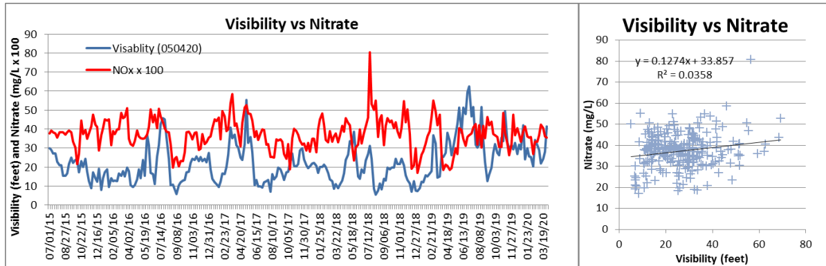
Figure 4.5: Weekly visibility and regression analysis at the spring boil and nitrate, 07/01/15 – 04/02/20. Visibility and nitrate by MLI.
